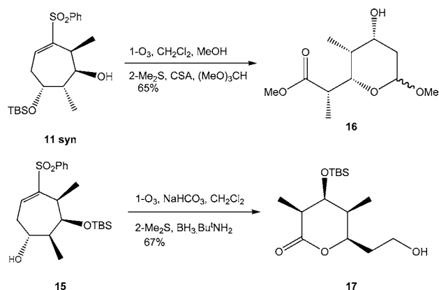
Scheme 5. Oxidative Cleavage of Vinyl Sulfone Stereotetrads
